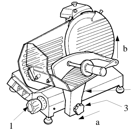
FIG. n°12 - Release of the carriage
